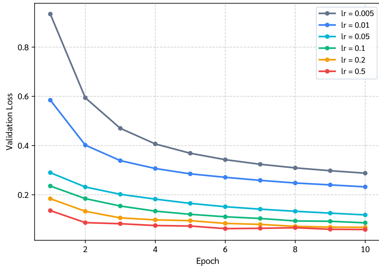
Validation Loss Trajectories Across Learning Rates (SGD)
