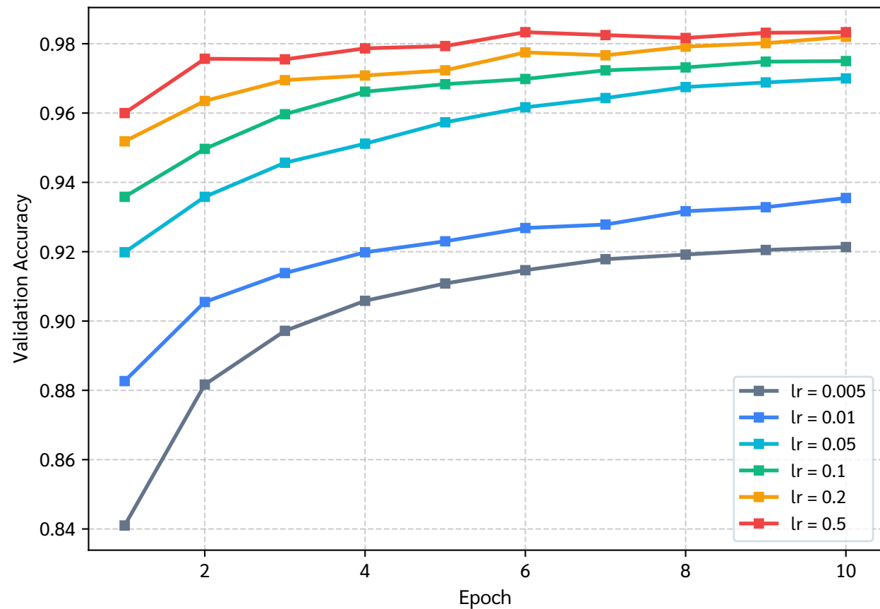
Validation Accuracy Dynamics Across Learning Rates (SGD)
